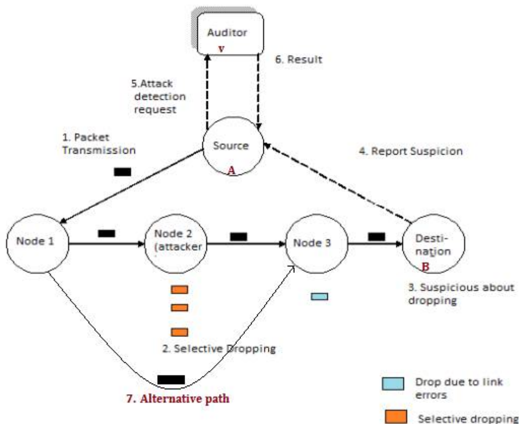
Fig 1. System Model
